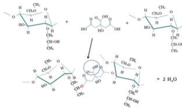
Figure 3 Schematic representation of esterification reaction between HPMC hydroxyl groups and citric acid [9]
