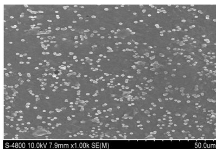
Figure 6 Papain particles distributed on the surface of HPMC hydrogel films by FESEM
